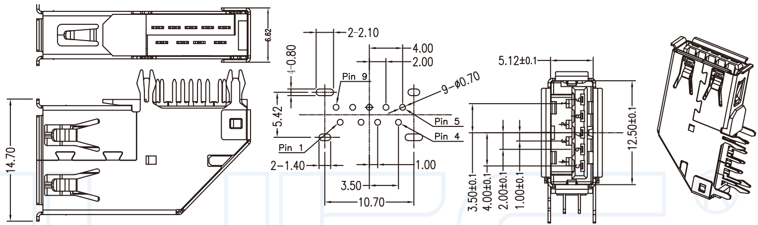
PCB LAYOUT (TOP VIEW) (TOLERANCE: ± 0.05)
