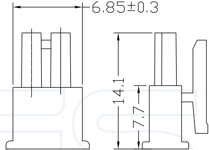
2P CIRCUIT HOUSING
