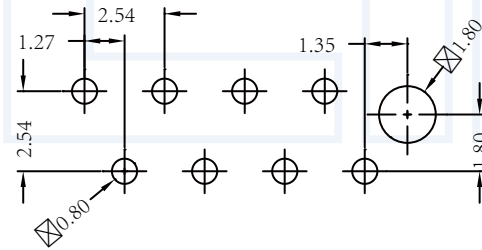
Recommended P.C.B Layout(Top Side)
