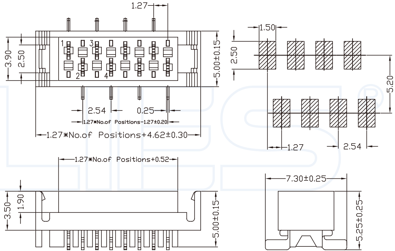
Recommended P.C.B Layout (Top Side)
